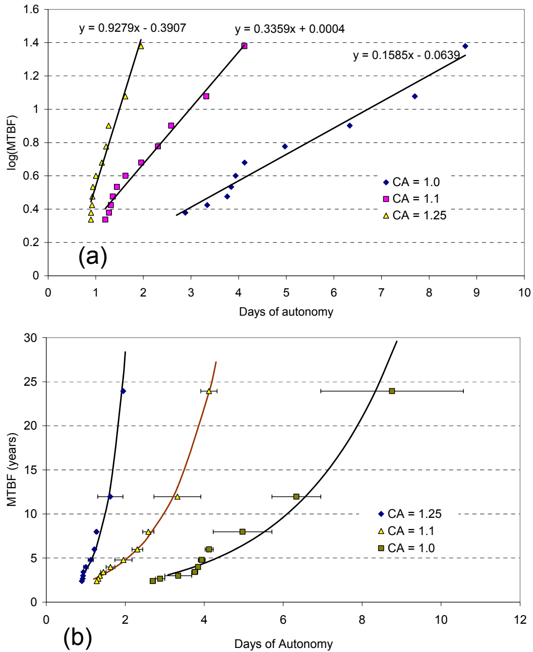
Fig. 2. An illustration of the method for fitting the dependence between the frequency of climatic cycles (interpreted as MTBF) and the required number of Days of Autonomy, on the example of WRDC data for Kumasi (Ghana). (a) The log-linear dependence, used to obtain the coefficient of the fit (Eq. (1)). (b) Actual dependence.
